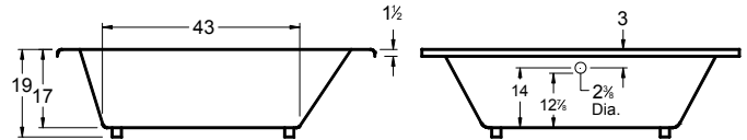
All bathtub dimensions are ± 1/2"
