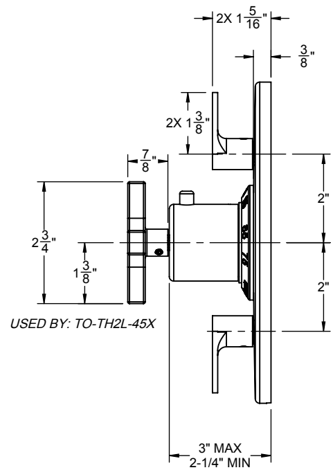
TO-TH2L-45X SHOWN
